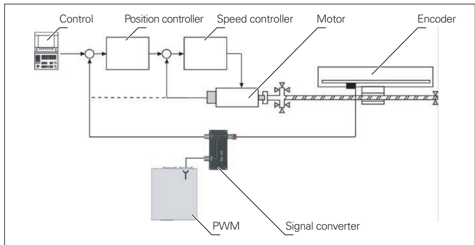
Monitoring mode with signal converter (potential segregation)
