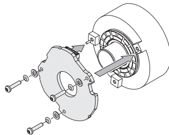
Mounting the scanning unit
