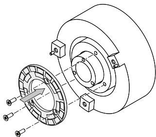
Screw-fastening the circular scale (Encoder B)
