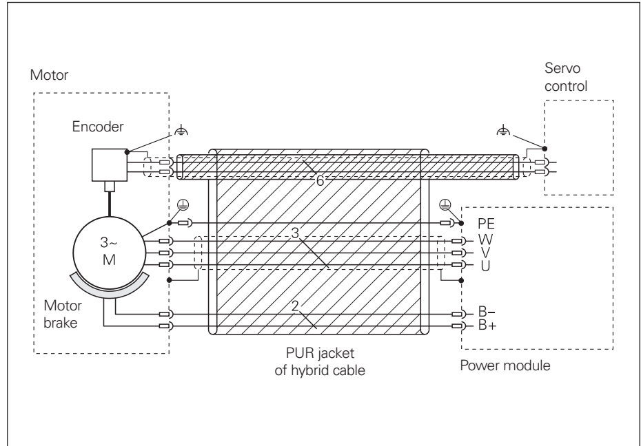
Grounding diagram
