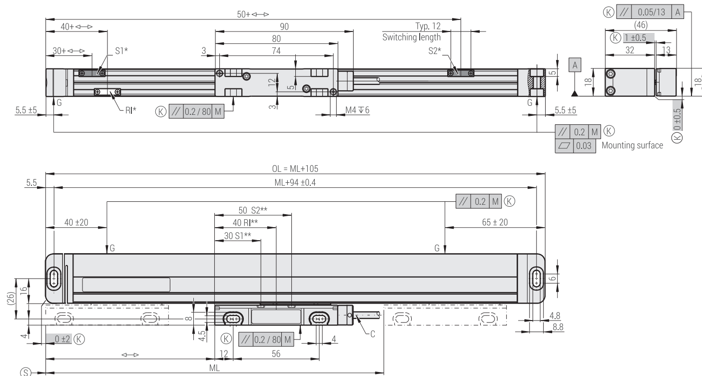
Dimensions, mounting tolerances MSA 830:
