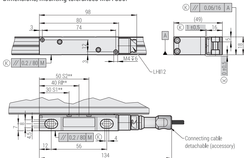
Dimensions, mounting tolerances MSA 830:
