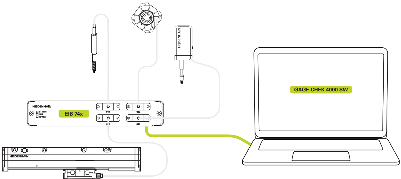
Connection of encoders through an EIB 74x
