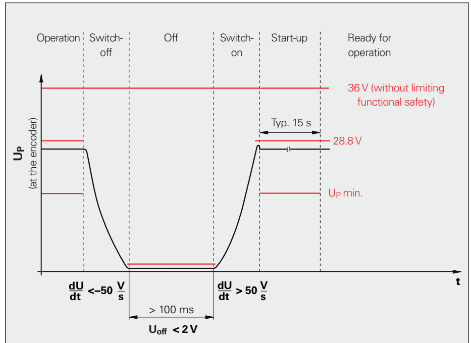
Switch-on/switch-off conditions for HEIDENHAIN encoders with the DRIVE-CLiQ interface
