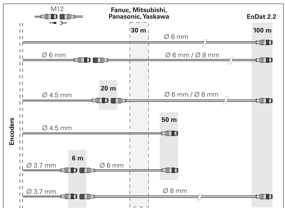
Cable lengths for purely serial interfaces
