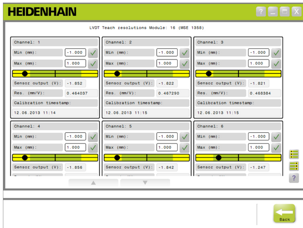
Scherm Resoluties inleren LVDT
