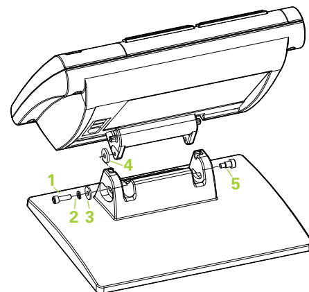
Stand assembly
